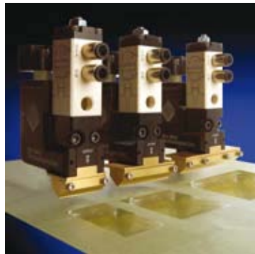
Slot Nozzles
